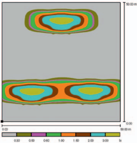
DIALUX Light intensity distribution curve (LID) Single- and double-view Example: pole distance 25 m
